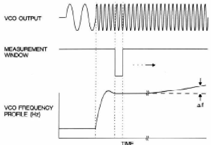
The flexible frequency profiling capability of the Phase Matrix 1230A/31A simplify VCO settling time and post tuning drift measurement.
